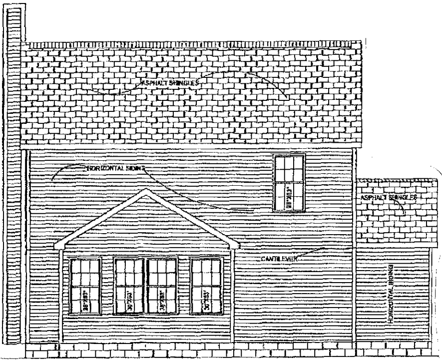
Sample Elevations for Oak Hollow Subdivision Cluster Lots
